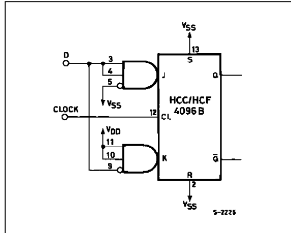
D-type Flip-Flop
