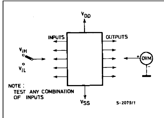
Noise Immunity.
