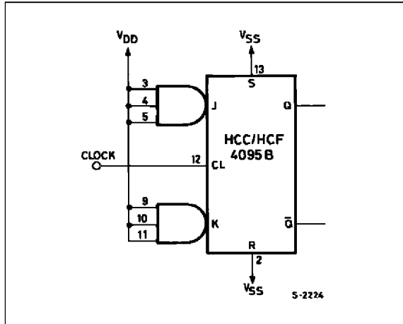
T-type Flip-Flop
