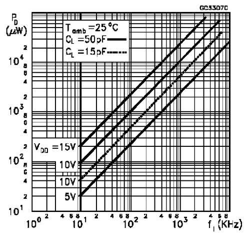
Typical Power Dissipation Per Gate vs Frequency
