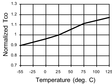
Normalized Tco vs Temp
