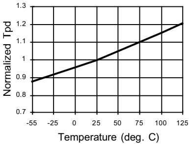
Normalized Tpd vs Temp
