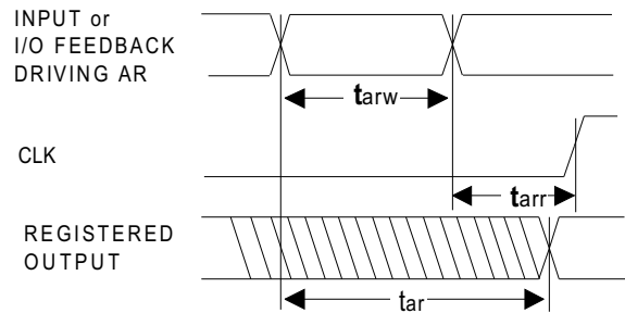
Asynchronous Reset
