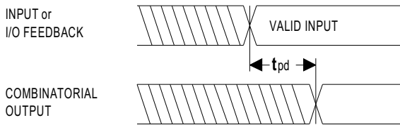
Combinatorial Output
