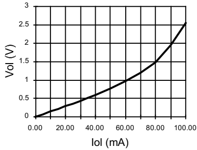
Vol vs Iol
