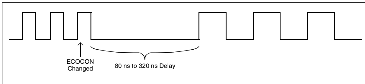
FIGURE 2-3: CLKOUT TRANSITION
