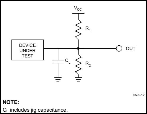
Figure 13. Test Configuration
