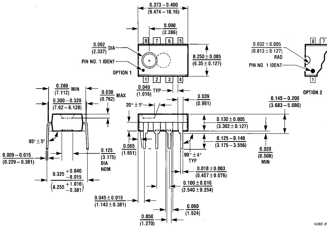
Molded Dual-In-Line Package (N) Order Number DS75451N, DS75452N, DS75453N NS Package Number N08E
