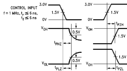
FIGURE 9. Load Enable and Disable Times for "LS-Type" Load
