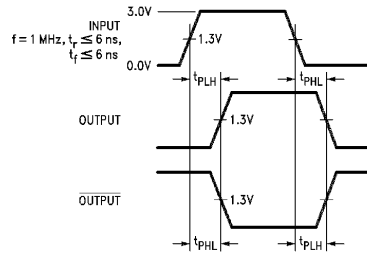
FIGURE 2. Propagation Delays
