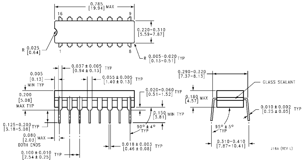
16-Lead Ceramic Dual-In-Line Package (J) Order Number DS34C87TJ NS Package Number J16A
