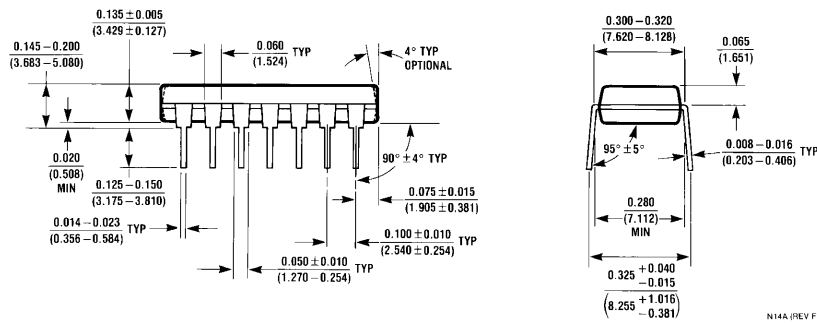
14-Lead Molded Dual-In-Line Package (N) Order Number DM74S20N NS Package Number N14A
