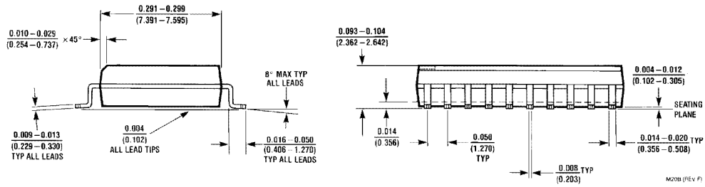
S.O. Package (M) Order Number DM64ALS374AWM, DM74ALS374AWM NS Package Number M20B
