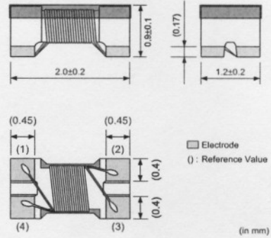
DLW21H Series
