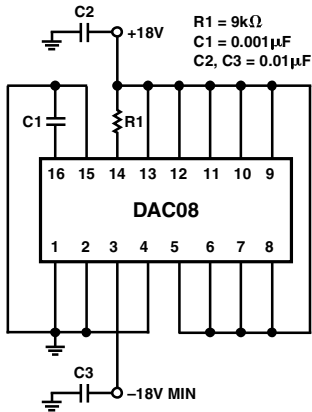
Figure 2. Burn-in Circuit
