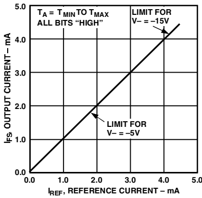
TPC 1. Full-Scale Current vs. Reference Current
