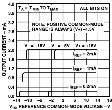
TPC 4. Reference Amp Common-Mode Range
