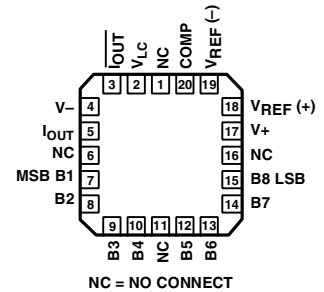
DAC08RC/883 20-Lead LCC (RC Suffix)
