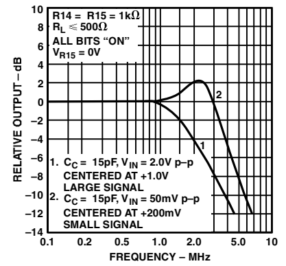
TPC 3. Reference Input Frequency Response
