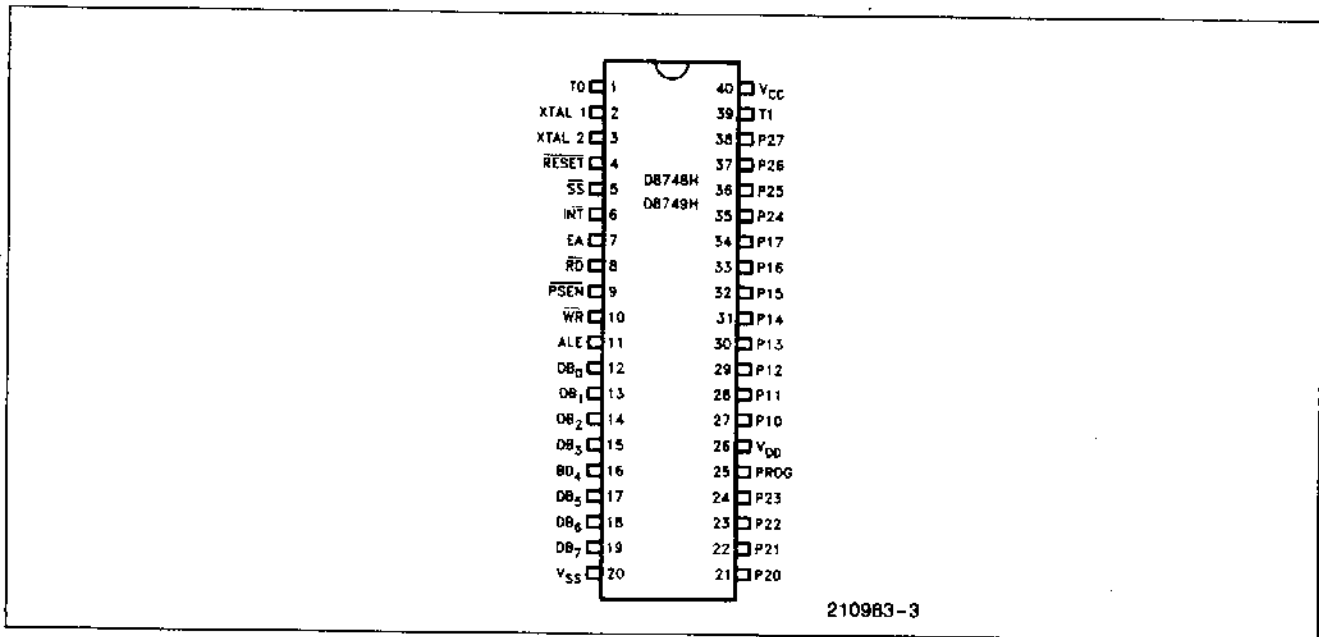
Figure 3. Pin Configuration
