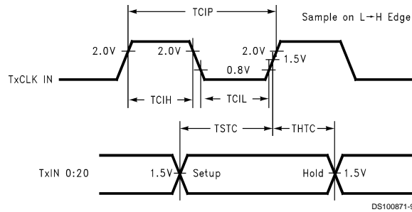
FIGURE 6. DS90CR217 (Transmitter) Setup/Hold and High/Low Times
