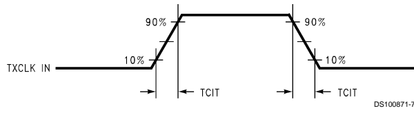
FIGURE 4. DS90CR217 (Transmitter) Input Clock Transition Time
