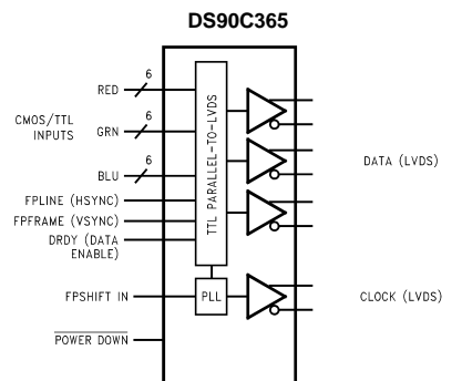
Order Number DS90C365MTD See NS Package Number MTD48
