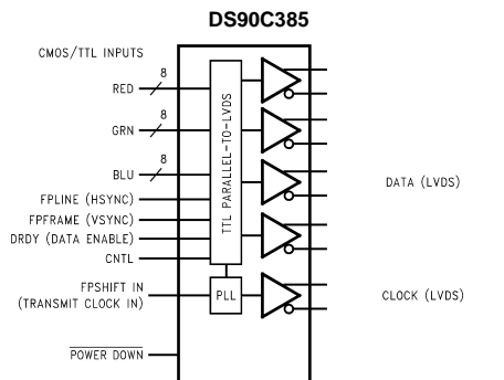
Order Number DS90C385MTD See NS Package Number MTD56
