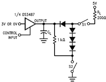
FIGURE 1. Propagation Delays
