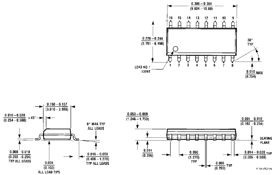
Small Outline Package (M) Order Number DS3487M NS Package Number M16A
