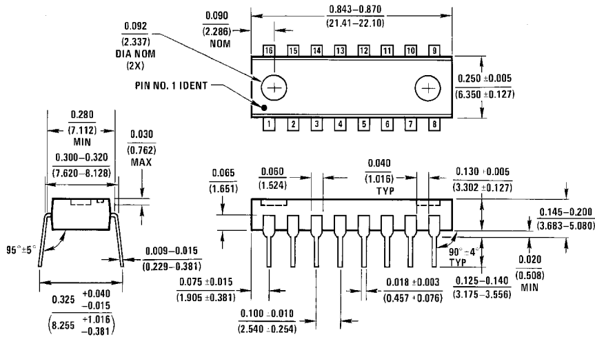
Molded Dual-In-Line Package (N) Order Number DS3487N NS Package Number N16A
