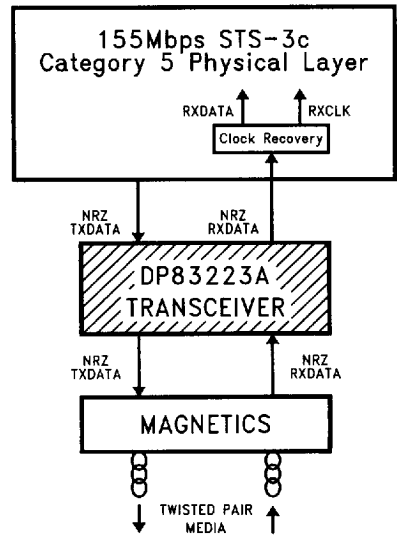
FIGURE 22. Typical STS-3c TP-ATM System Connection
