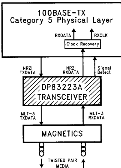
FIGURE 21. Typical 100BASE-TX System Connection
