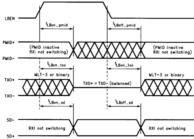
FIGURE 29. Loopback Timing
