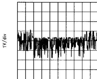
FIGURE 4. Baseline Wander Event
