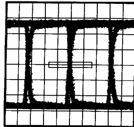
FIGURE 15. Recovered ECL Peak Total Jitter for 50M of CAT-5 Cable (binary) 480 ps
