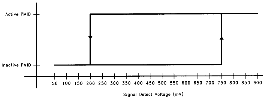
FIGURE 17. Signal Detect
