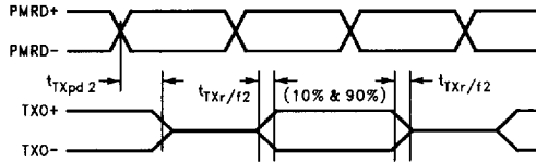
FIGURE 26. TXO Timing (MLT-3)
