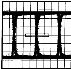
FIGURE 16. Recovered ECL Peak Total Jitter for 100M of CAT-5 Cable (binary) 520 ps
