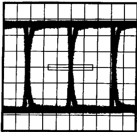
FIGURE 14. Recovered ECL Peak Total Jitter for 0M of CAT-5 Cable (binary) 340 ps
