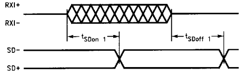
FIGURE 32. Signal Detect Timing (Binary RXI to SD)
