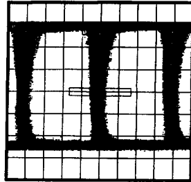
FIGURE 13. Recovered ECL Peak Total Jitter for 100M of CAT-5 Cable (MLT-3) 1.08 ns
