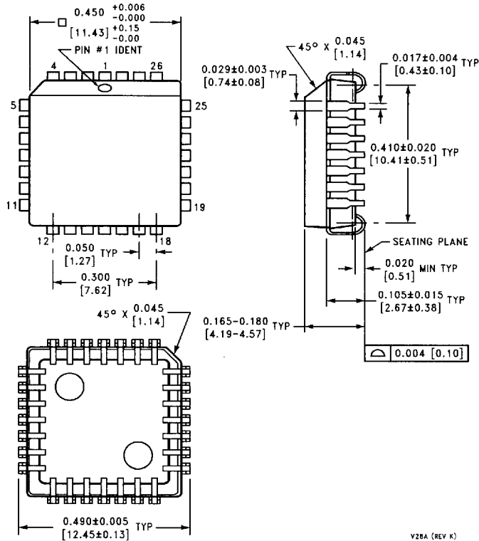
Plastic Lead Chip Carrier (V) Order Number DP83223AV NS Package Number V28A
