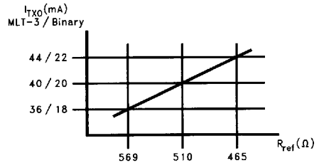
FIGURE 24b. Typical TXO Current vs R_{\text{REF}}
