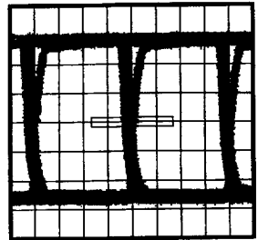
FIGURE 9. Recovered ECL Peak Total Jitter for 0M of CAT-5 Cable (MLT-3) 660 ps
