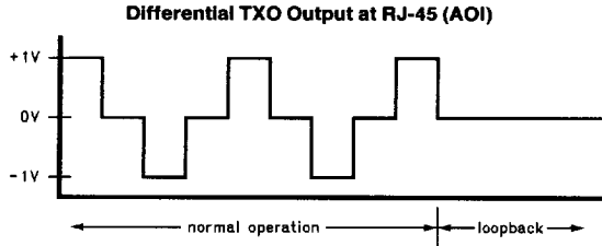
FIGURE 18. TXO True Quiet during Loopback (MLT-3 Mode)
