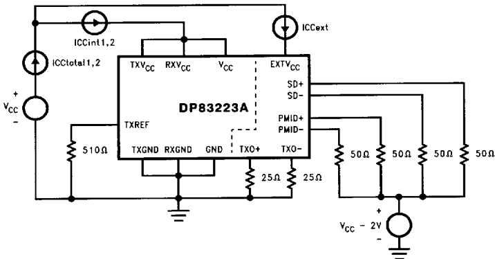
FIGURE 24c. ICc Diagram
