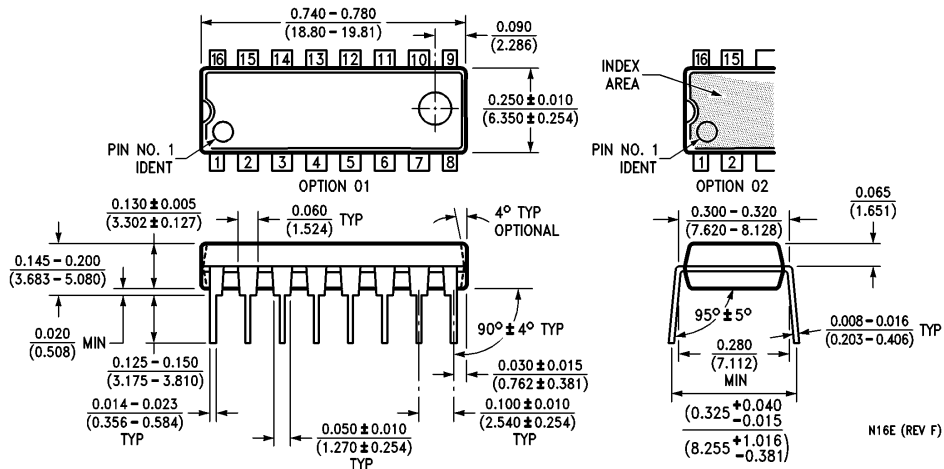
16-Lead Molded Dual-In-Line Package (N) Order Number DM74S138N or DM74S139N NS Package Number N16E
