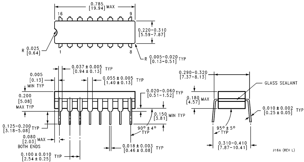
16-Lead Ceramic Dual-In-Line Package (J) Order Number DM54S138J or DM54S139J NS Package Number J16A
