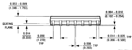
14-Lead Small Outline Molded Package (M) Order Number DM74S05M NS Package Number M14A
