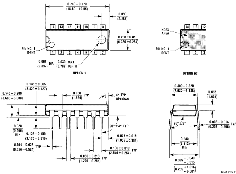
14-Lead Molded Dual-In-Line Package (N) Order Number DM74S05N NS Package Number N14A
