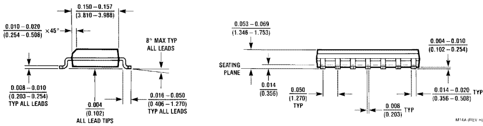
14-Lead Small Outline Molded Package (M) Order Number DM74LS03M NS Package Number M14A
