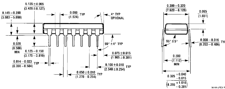
14-Lead Molded Dual-In-Line Package (N) Order Number DM74LS03N NS Package Number N14A
