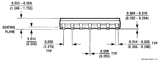
S.O. Package (M) Order Number DM74ALS74AM NS Package Number M14A
