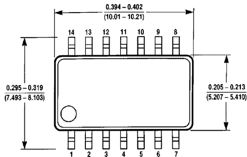
S.O. Package (M) Order Number DM74ALS74AM NS Package Number M14A
