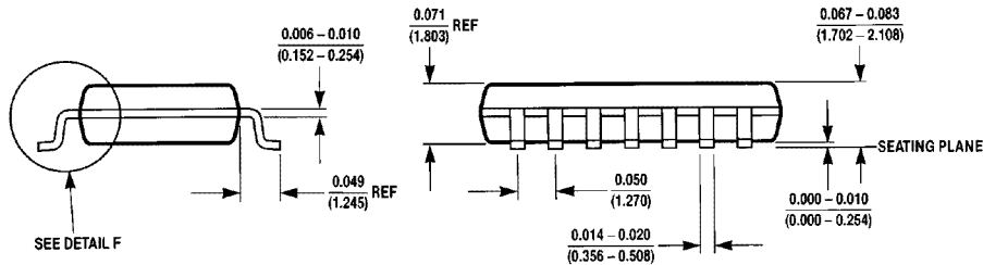
Small Outline Package (SJ) Order Number DM74ALS74ASJ NS Package Number M14D
