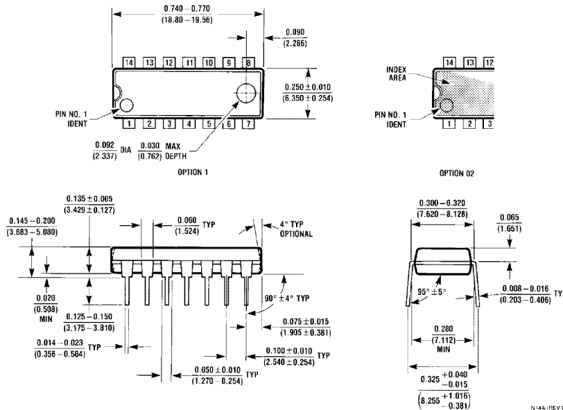
Molded Dual-In-Line Package (N) Order Number DM74ALS20AN NS Package Number N14A
