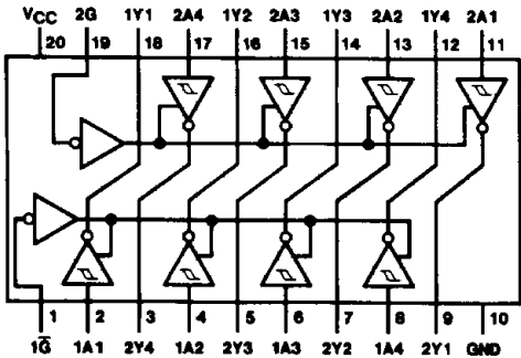
TL/F/6478-1
