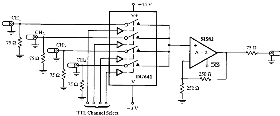
Figure 8. 4 by 1 Video Multiplexing Using the DG641
