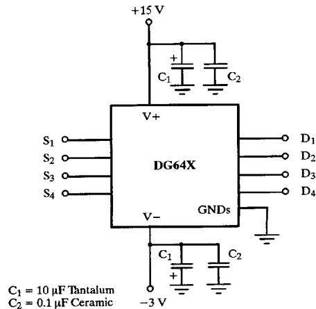
Figure 7. Supply Decoupling
