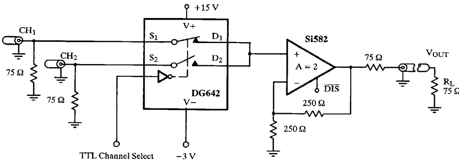
Figure 9. 2-Channel Video Selector Using the DG642
