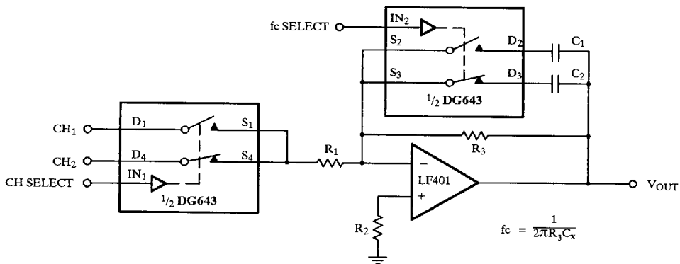
Figure 10. Active Low Pass Filter with Selectable Inputs and Break Frequencies
