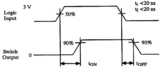
Figure 2. Switching Time
