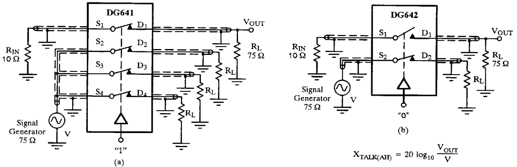
Figure 5. All Hostile Crosstalk - X_{TALK(AH)}
