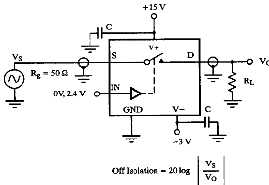
Figure 4. Off Isolation
