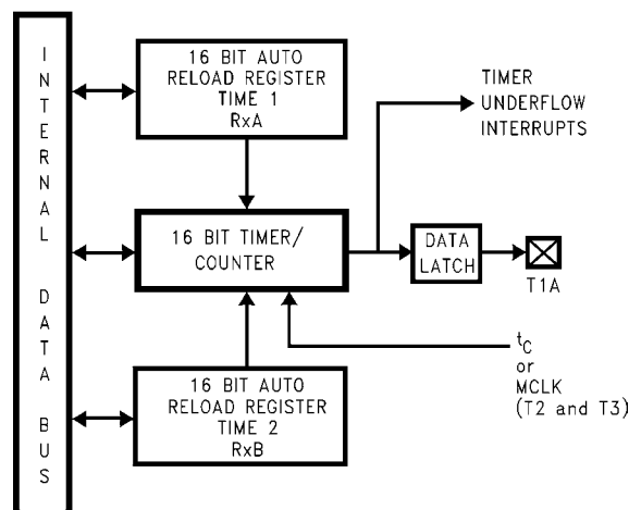
FIGURE 16. Timer in PWM Mode
