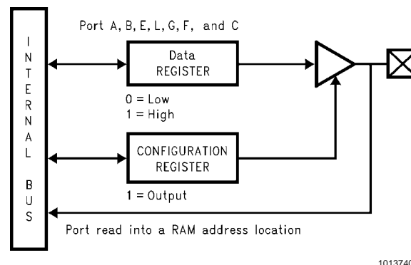
FIGURE 4. I/O Port Configurations—Output Mode
