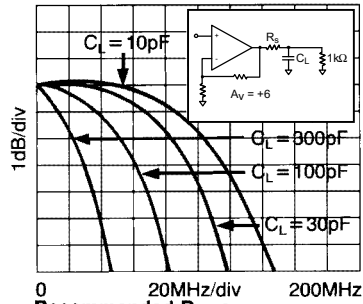
Recommended R_s vs Load Capacitance
