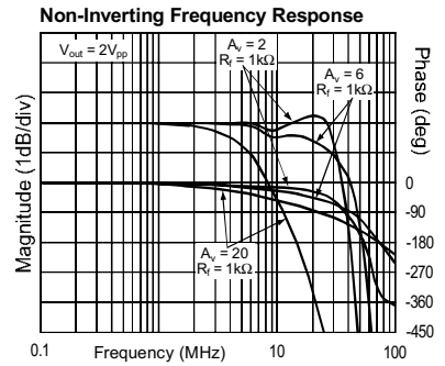
I_{CC} = 1mA, R_L = 1000\Omega
