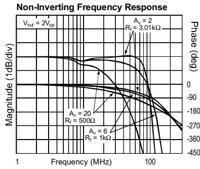
I_{CC} = 3.4mA, R_L = 500\Omega
