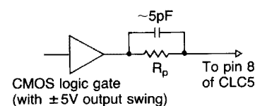
Figure 3: dynamic control of power consumption
