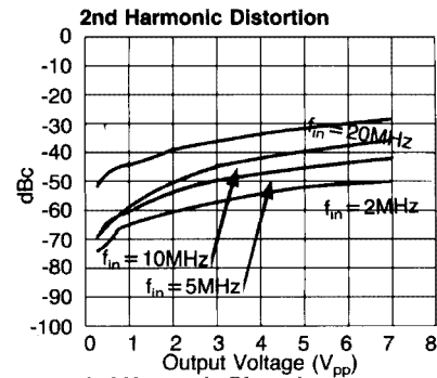
I_{CC} = 1mA , R_L = 1000\Omega
