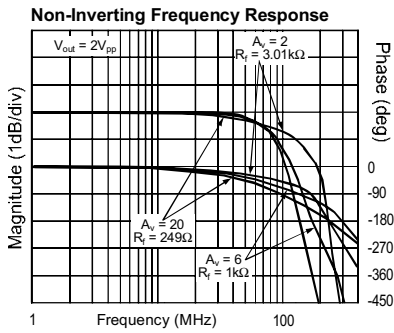
I_{CC} = 9mA, R_L = 250\Omega
