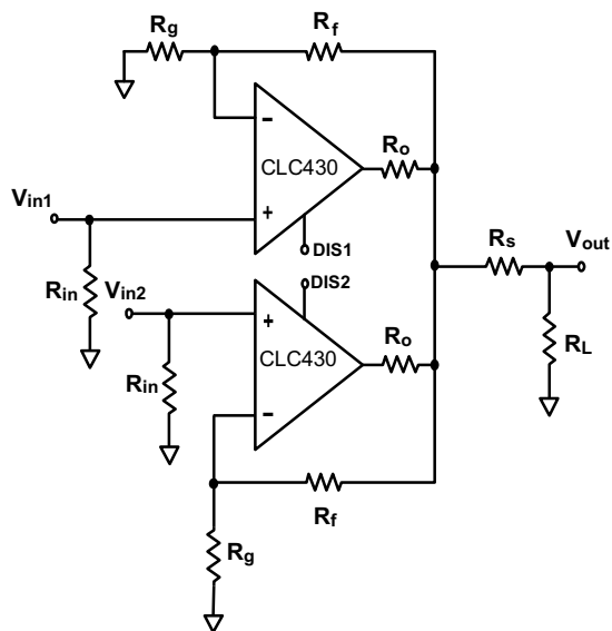
FIGURE 6. Output Connection
