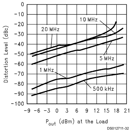
2nd Harmonic Distortion vs. P OUT
