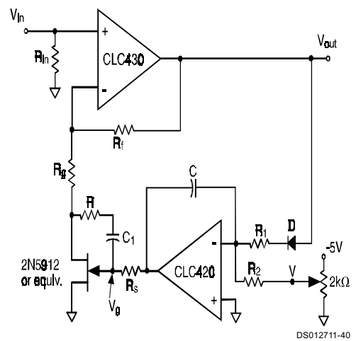
FIGURE 7. AGC Circuit
