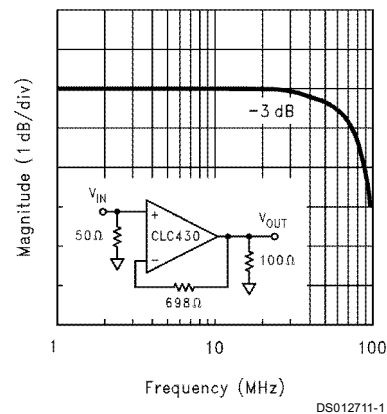
Unity-Gain Frequency Response
