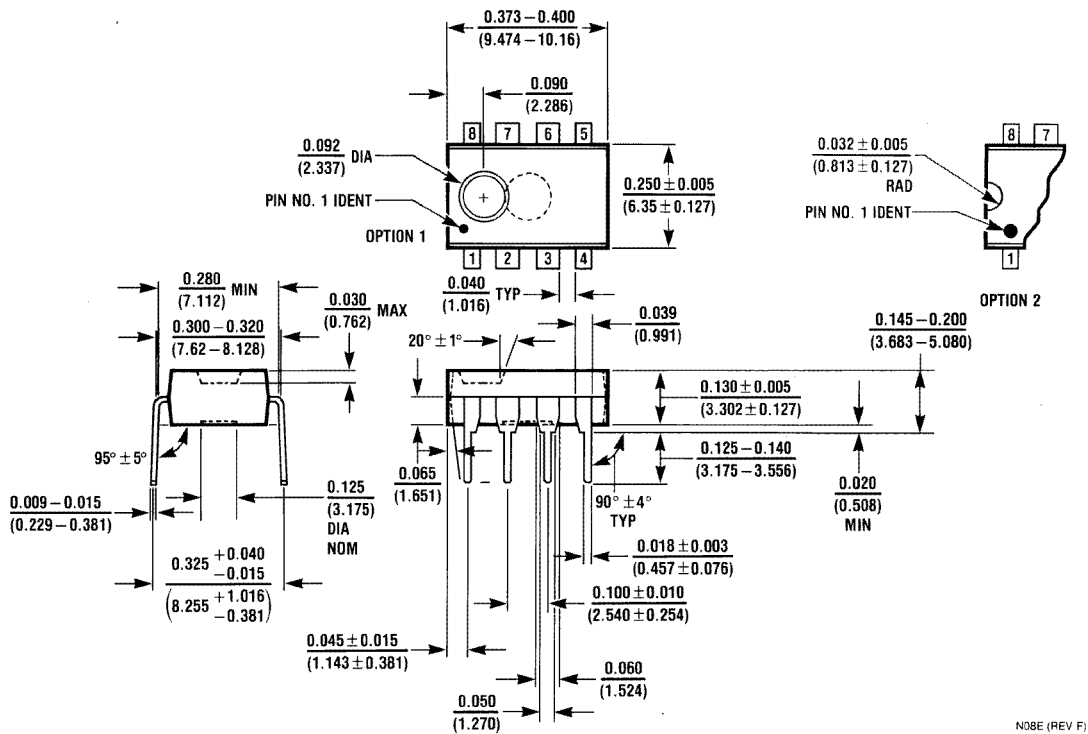
8-Pin MDIP NS Product Number N08E
