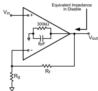
FIGURE 3. Equivalent Disabled Output Impedance
