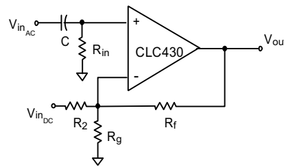
FIGURE 5. Level Shifting Circuit
