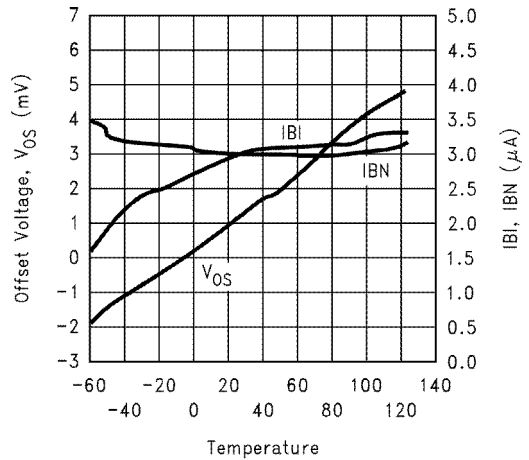
Typical I_{BI} , I_{BN} , V_{OS} vs. Temperature
