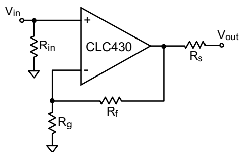
FIGURE 1. Component Identification
