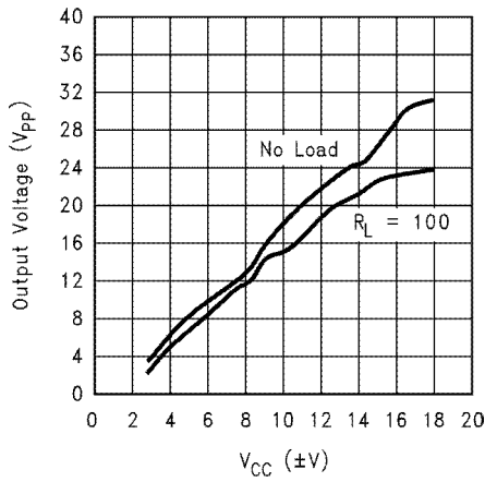
Maximum Output Voltage vs. V_{CC}
