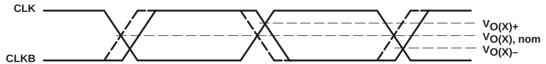
Figure 6. Crossing-Point Voltage
