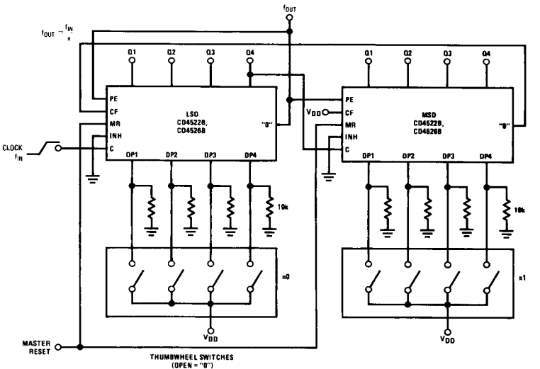
2-Stage Programmable Frequency Divider
