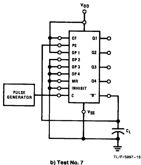
FIGURE 1. Test Circuits
