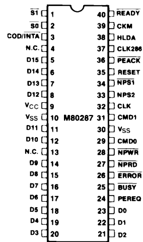
Figure 2. M80287 Pin Configuration
