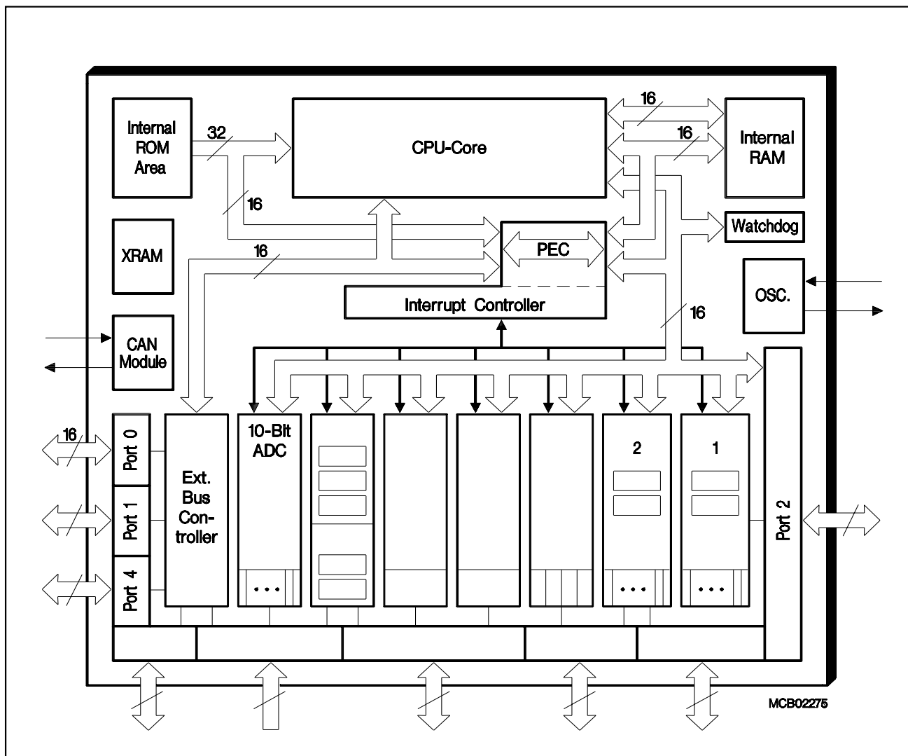
Figure 3 Block Diagram
