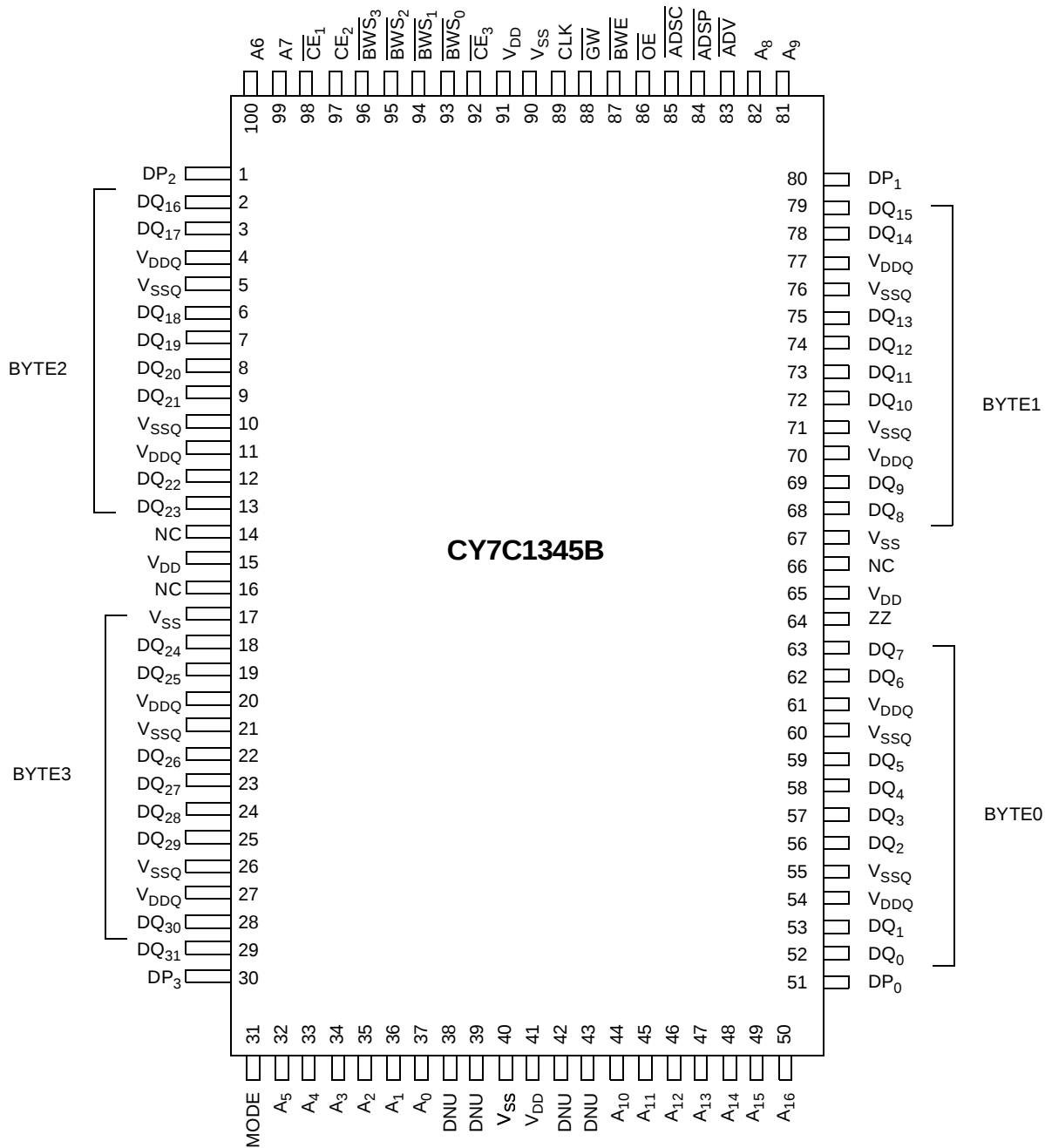
100-Pin TQFP
