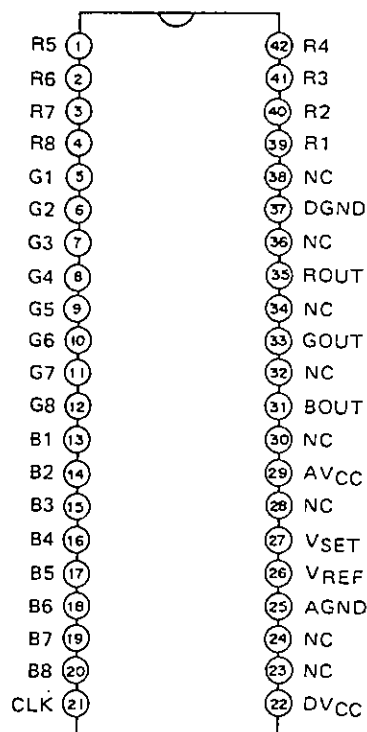
Pin Configuration (Top View)
