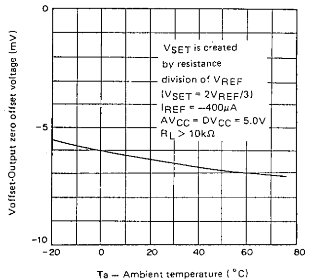
Output zero offset voltage vs. Ambient temperature
