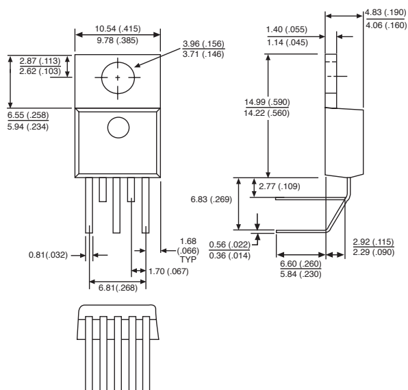
5 Lead TO-220 (TVA) Vertical
