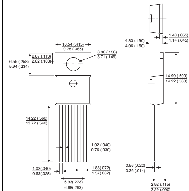
5 Lead TO-220 (T) Straight
