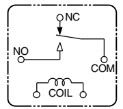
Schematic (Top view)
