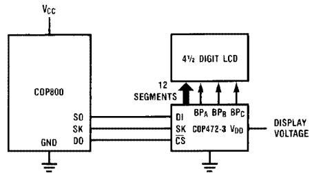
FIGURE 6. System Diagram – 4½ Digit Display
