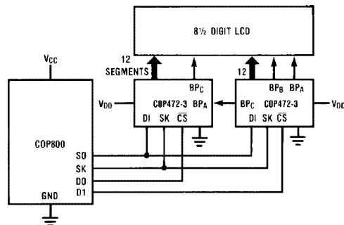
FIGURE 7. System Diagram – 8½ Digit Display
