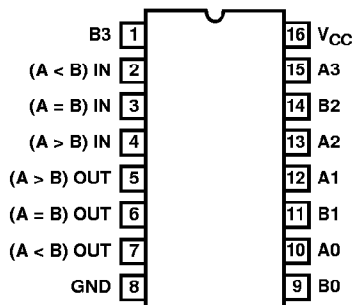
CD74HC85, CD74HCT85 (PDIP, SOIC) TOP VIEW
