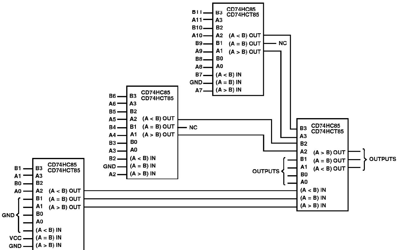
FIGURE 4. PARALLEL CASCADING - COMPARING 12-BIT WORDS
