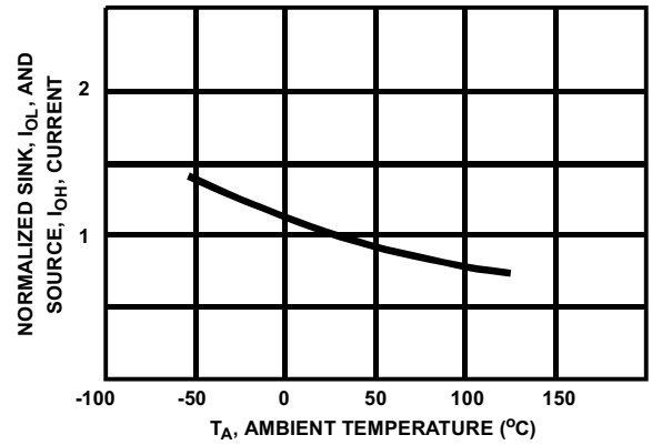
FIGURE 11. VARIATION OF NORMALIZED OUTPUT LOW (SINK) CURRENT I_{OL} AND OUTPUT HIGH (SOURCE) CURRENT I_{OH} WITH TEMPERATURE
