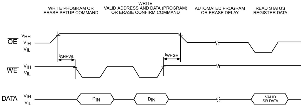
Figure 8. Alternate Boot Block Access Method Using OE
