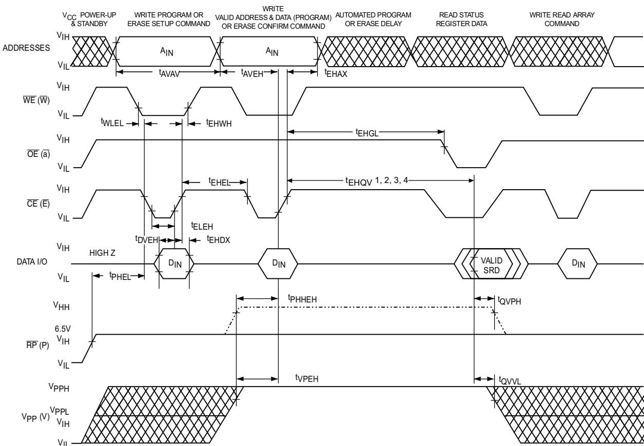
Figure 9. Alternate AC Waveform for Write Operations
