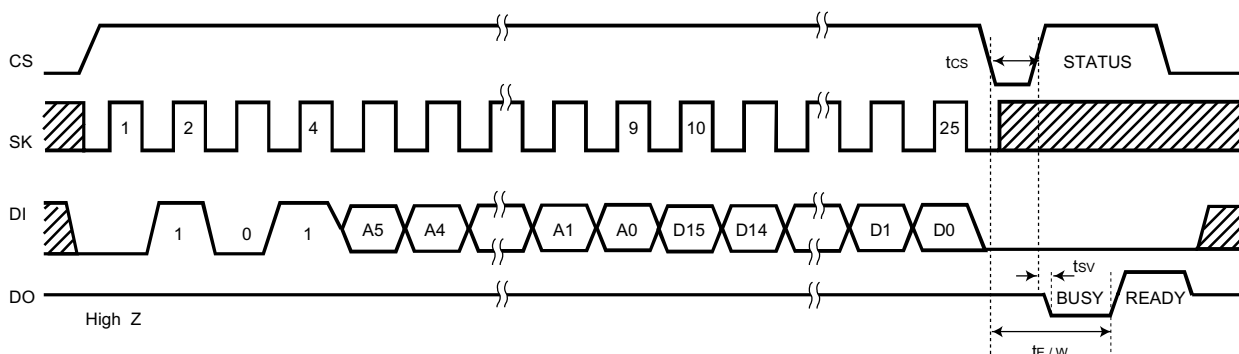
Fig. 4 Write cycle timing (WRITE)
