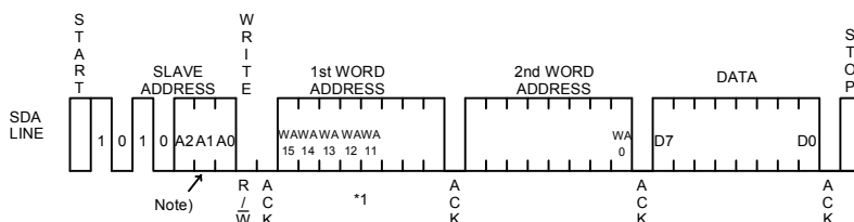
Fig.39 Byte write cycle (BR24T32/64/128/256/512/1M-W)
