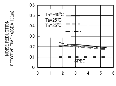
Fig.32 Noise reduction effective time t_t(SDA H)
