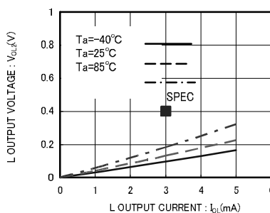
Fig.6 'L' output voltage V_{OL} ( V_{CC}=2.5V )
