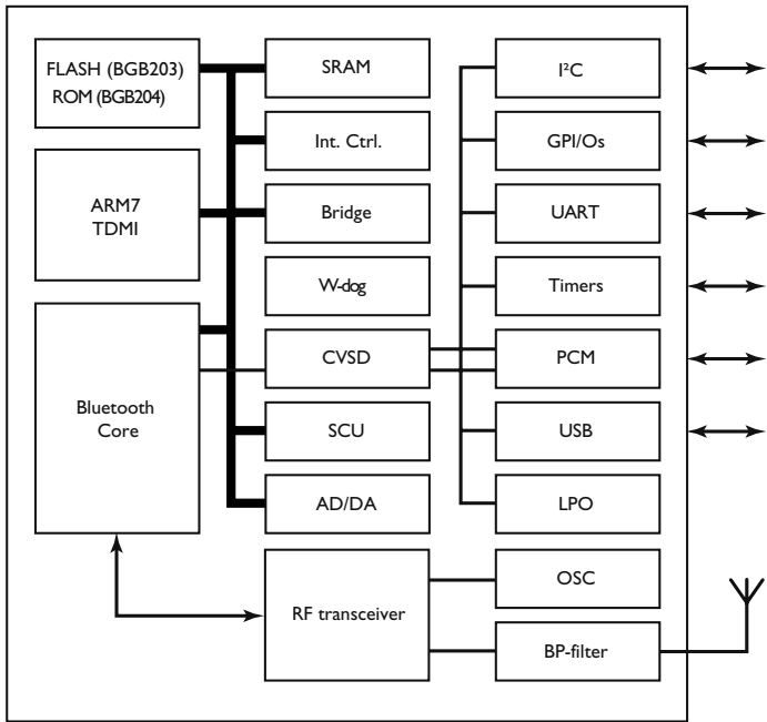
BGB210 functional block diagram
