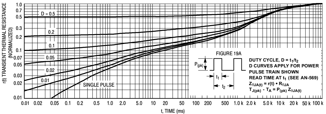
Figure 16. Thermal Response
