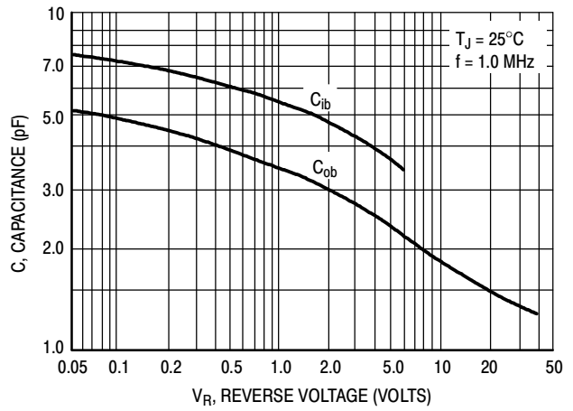
Figure 15. Capacitance
