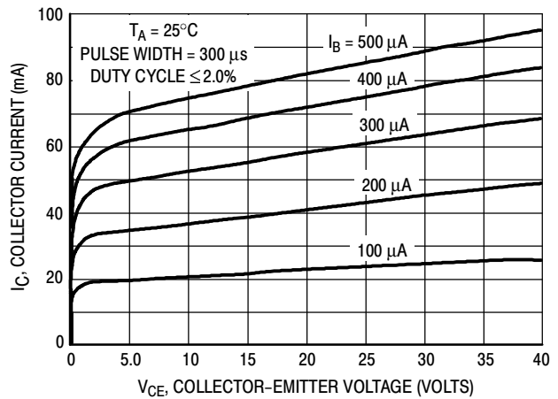
Figure 9. Collector Characteristics
