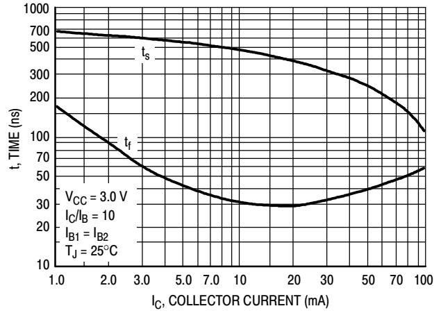
Figure 13. Turn-Off Time
