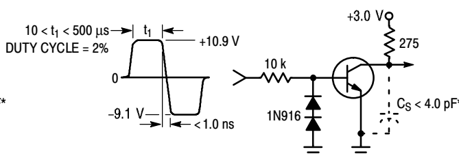
Figure 2. Turn-Off Time
