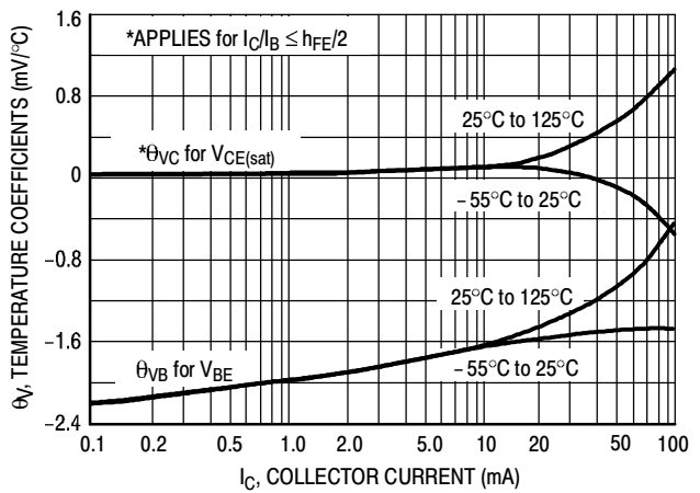
Figure 11. Temperature Coefficients
