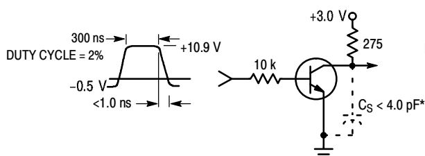
Figure 1. Turn-On Time
