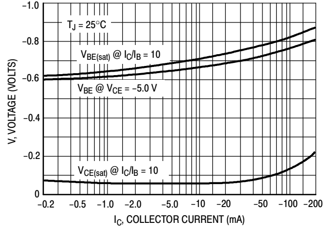
Figure 8. "On" Voltage
