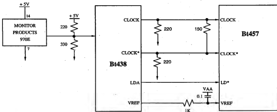
Figure 6. Generating the Bt457 Clock Signals (Monochrome Application).
