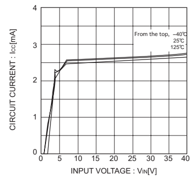
Fig.6 Circuit current (BD9781HFP)
