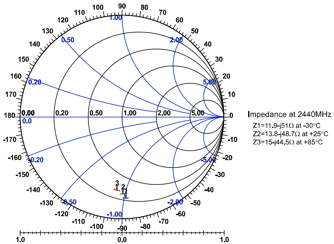
Figure 9.10: RX_B Balanced
