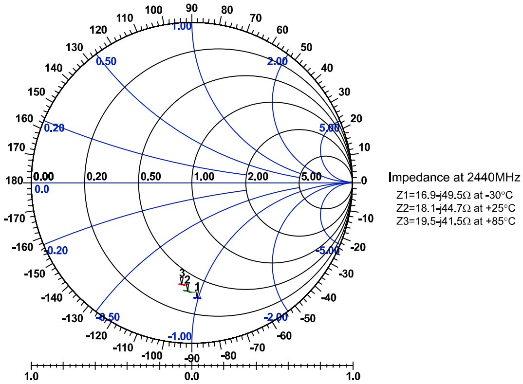
Figure 9.3: TX_A PL35
