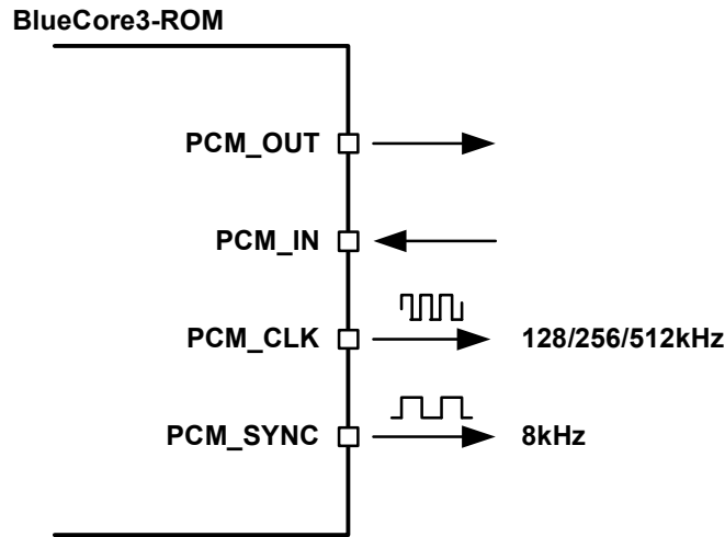
Figure 9.27: BlueCore3-ROM as PCM Interface Master
