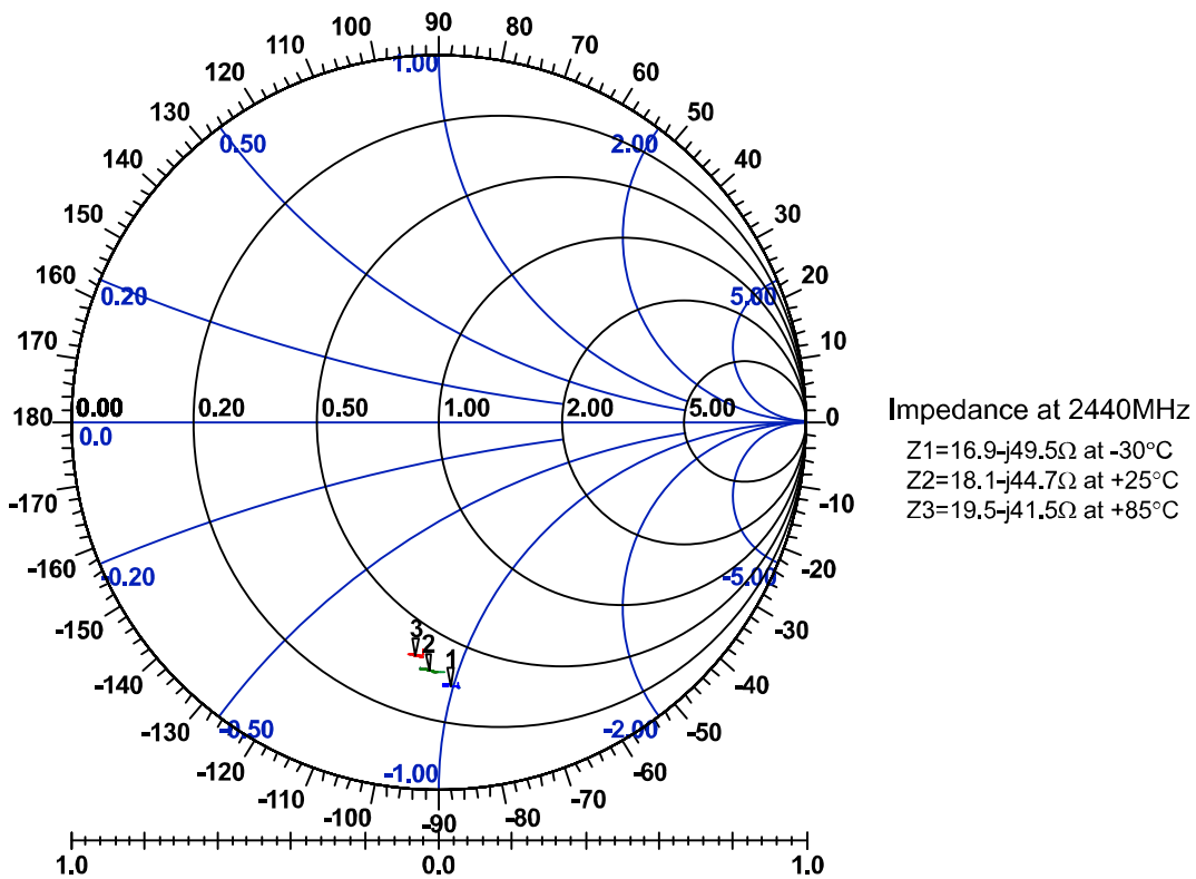
Figure 9.4: TX_A PL50
