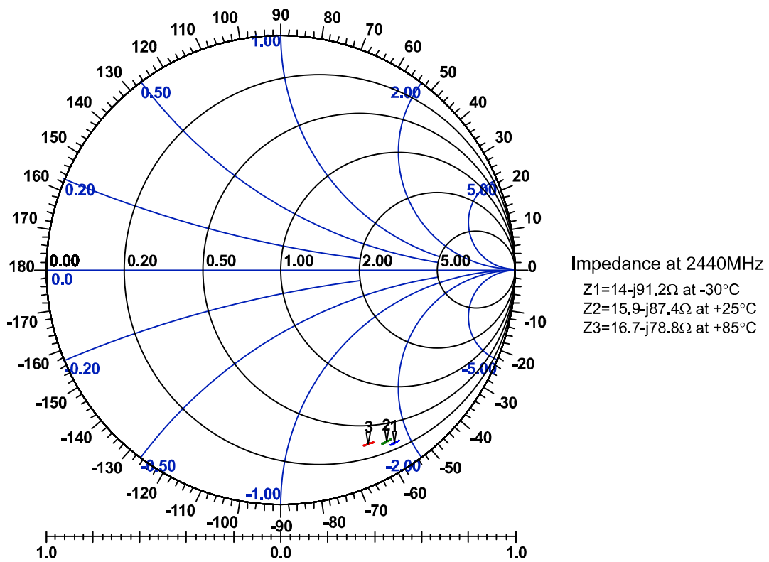
Figure 9.11: RX Un-Balanced
