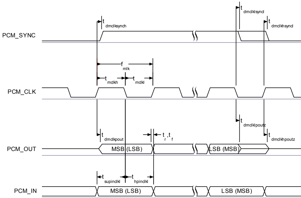
Figure 9.34: PCM Master Timing Long Frame Sync
