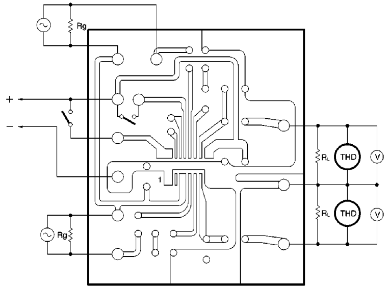
(Printed circuit)
