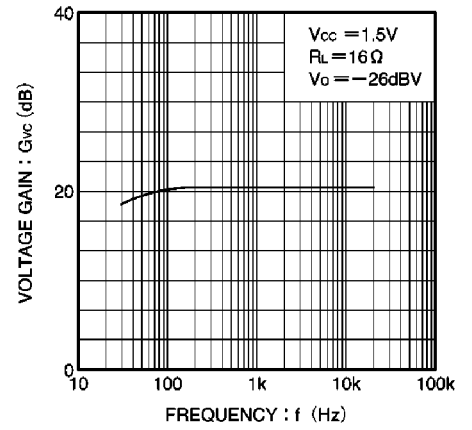
Fig. 15 Voltage gain vs. frequency
