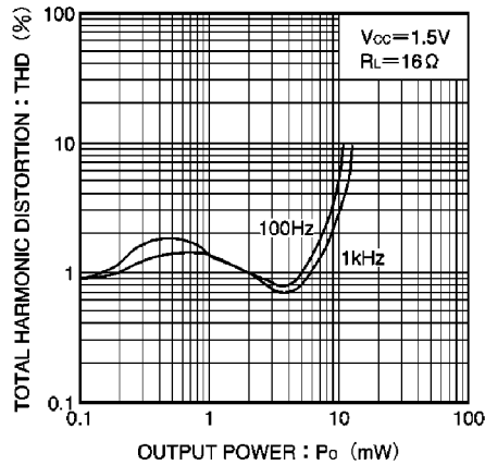
Fig. 17 Total harmonic distortion vs. output voltage
