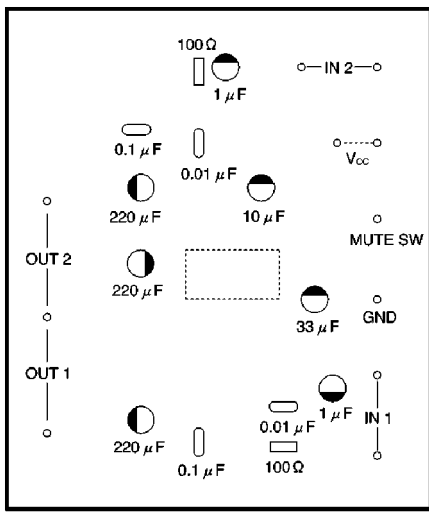
(Components)
