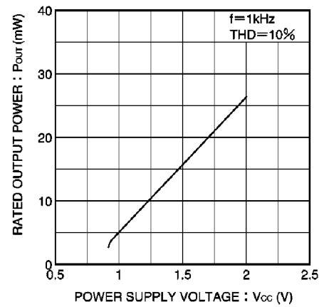
Fig. 12 Output voltage vs. power supply voltage
