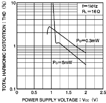
Fig. 16 Total harmonic distortion vs. power supply voltage
