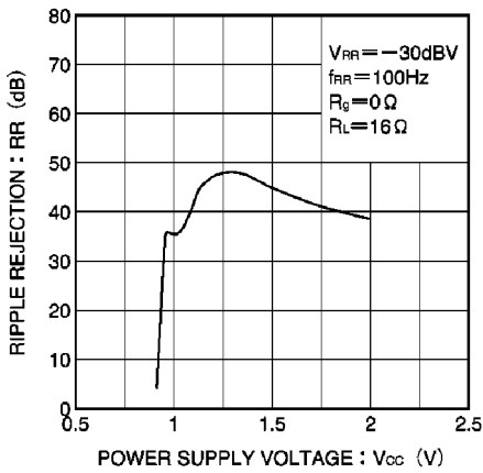
Fig. 13 Ripple rejection ratio vs. power supply voltage
