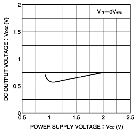
Fig. 11 DC output voltage vs. power supply voltage
