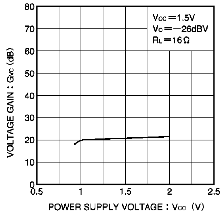
Fig. 14 Voltage gain vs. power supply voltage
