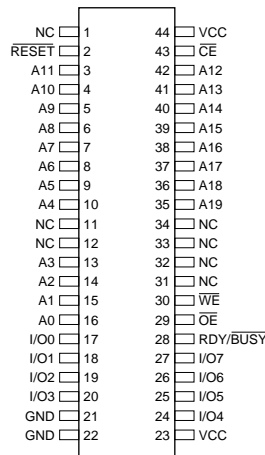
TSOP Top View Type 1
