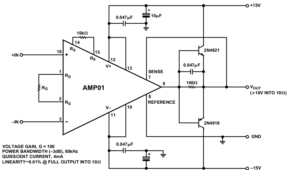
Figure 38. Adding Two Transistors Increases Output Current to \pm 1 A Without Affecting the Quiescent Current of 4 mA. Power Bandwidth is 60 kHz.
