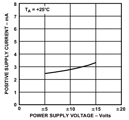
Figure 25. Positive Supply Current vs. Supply Voltage
