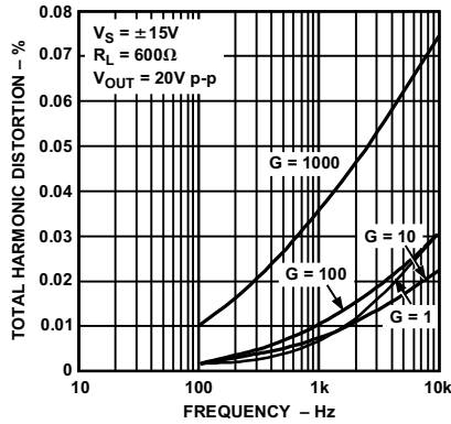
Figure 18. Total Harmonic Distortion vs. Frequency
