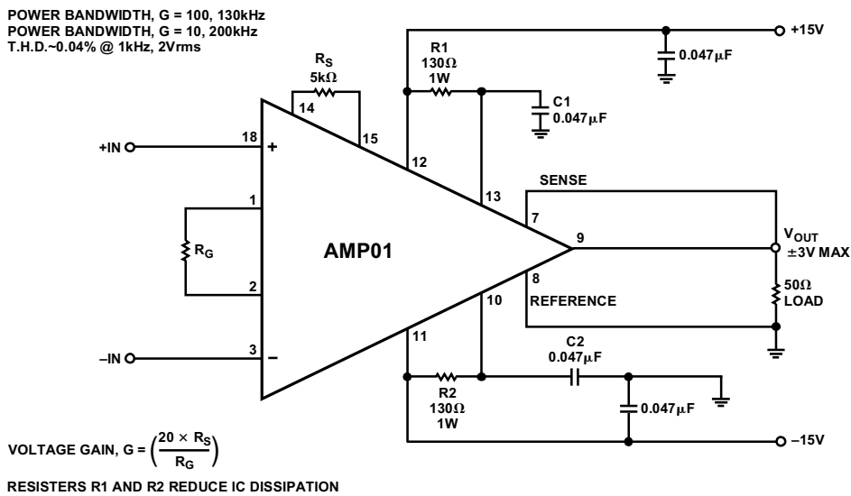
Figure 34. Driving 50 Ω Loads
