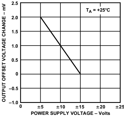
Figure 5. Output Offset Voltage Change vs. Supply Voltage
